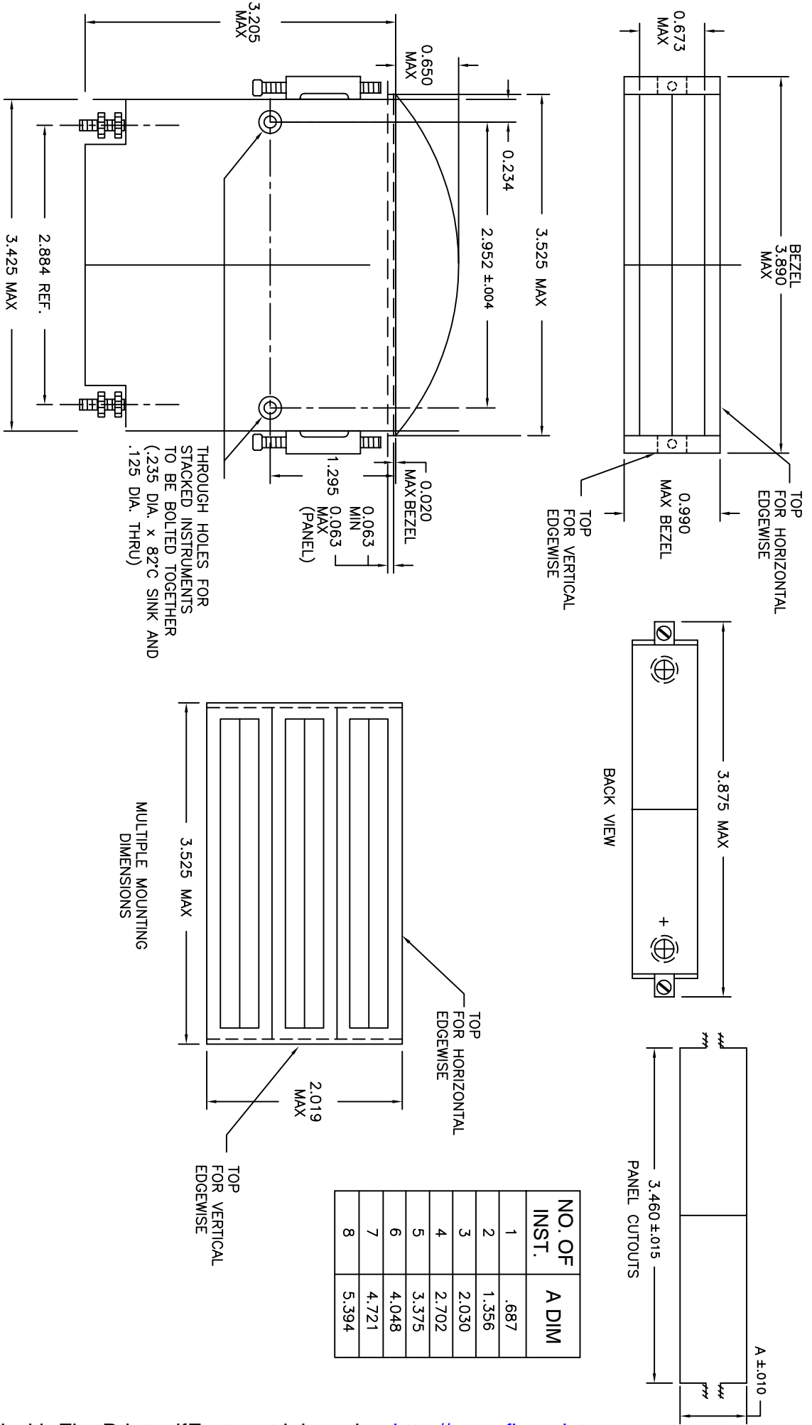
FIG. 19. OUTLINE DIMENSIONS FOR 3 1/2 INCH TYPE 288 METERS REV 1/22/03 (DWG 3151K78)
